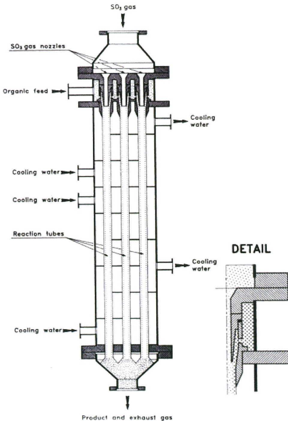
FIG. 9 Multitube film reactor (Ballestra).
